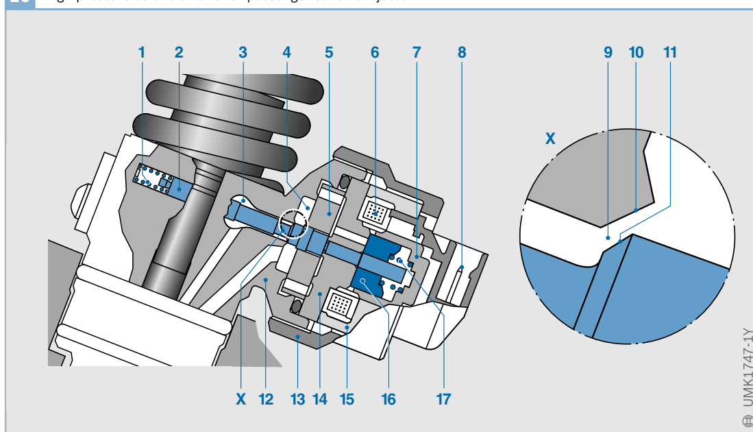
10 High-pressure solenoid valve for passenger-car unit injector
