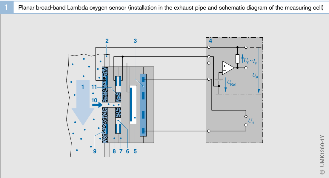
Fig. 1 1 Exhaust gas 2 Exhaust pipe 3 Heater 4 Control electronics 5 Reference cell with reference-air passage 6 Diffusion gap 7 Nernst concentration cell 8 Oxygen-pump cell with pump electrode 9 Porous protective layer 10 Gas-access passage 11 Porous diffusion barrier
