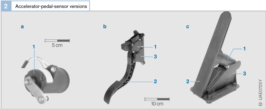
Fig. 2 a Individual accelerator-pedal sensor b Top-mounted accelerator-pedal module c Bottom-mounted accelerator-pedal module FMP1 1 Sensor 2 Vehicle-specific pedal 3 Pedal bracket
