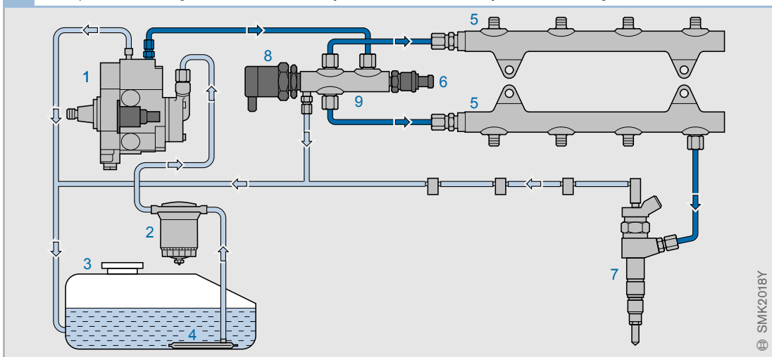
2 Example of a second-generation common-rail system with two-actuator system for a V8 engine
