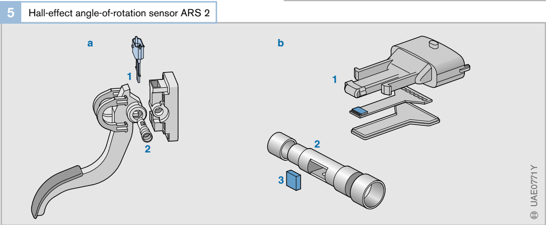
Fig. 5 a Installation in the accelerator-pedal module b Components 1 Hall-effect sensor 2 Pedal shaft 3 Magnet
