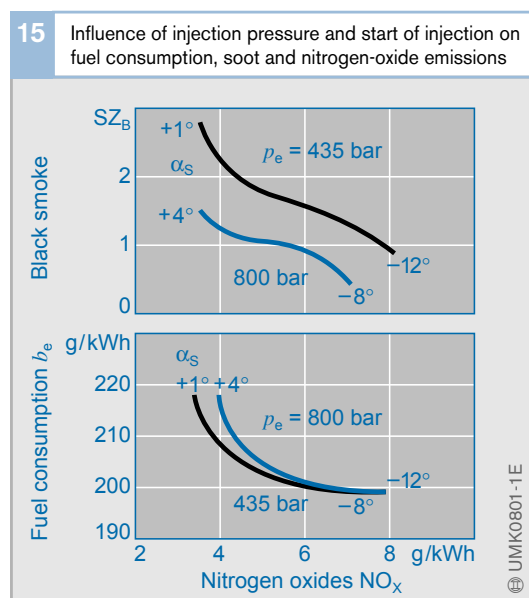
Fig. 15 Direct-injection engine, engine speed 1,200 rpm, mean pressure 16.2 bar
