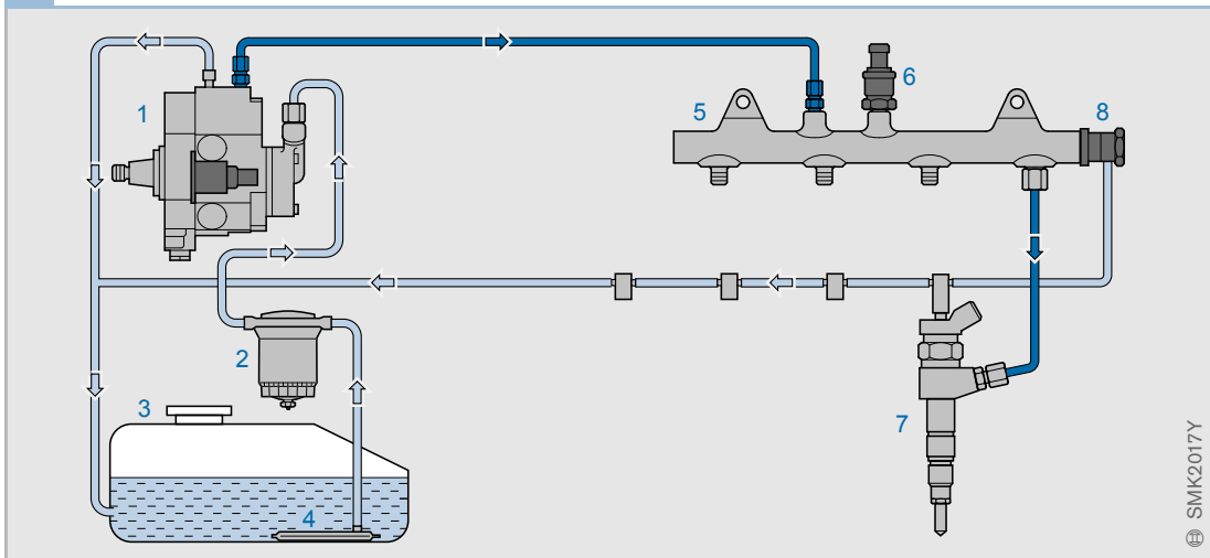
1 Example of a second-generation common-rail system for a 4-cylinder engine
