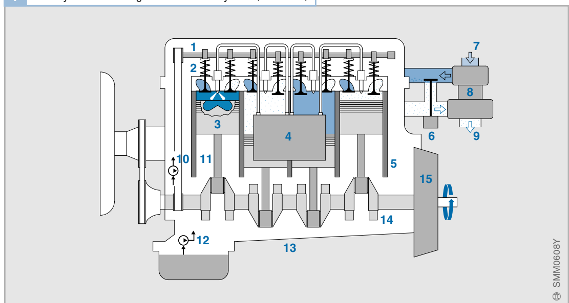
1 Four-cylinder diesel engine without auxiliary units (schematic)
