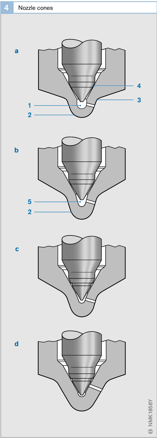
Fig. 4 a Cylindrical blind hole and conical tip a Conical blind hole and conical tip c Micro-blind-hole d Sac-less (vco) nozzle 1 Cylindrical blind hole 2 Conical tip 3 Neck radius 4 Nozzle-body seat face 5 Conical blind hole
