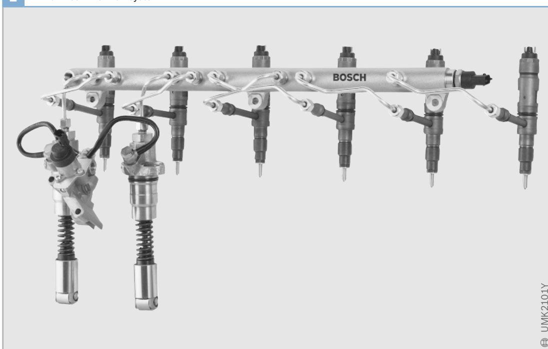
2 PF 45 in common-rail system
