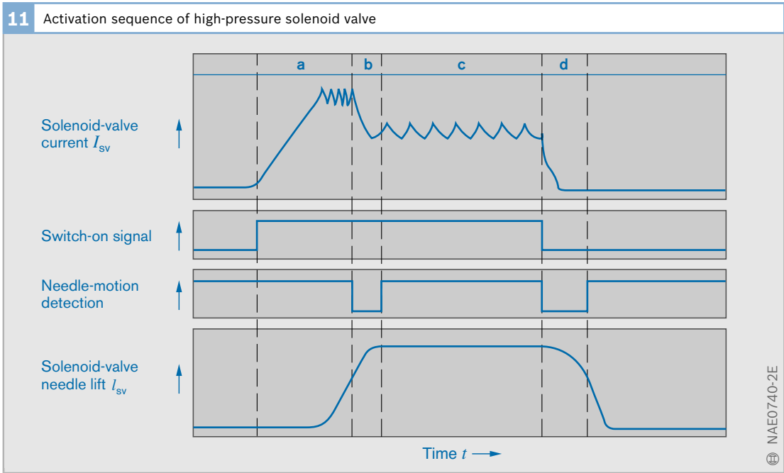
Fig. 11 a Pickup current (commercial-vehicle UIS/UPS: 12...20 A; passenger-car UIS: 20 A) b BIP detection c Holding current (commercial-vehicle UIS/UPS: 8...14 A; passenger-car UIS: 12 A) d High-speed quenching
