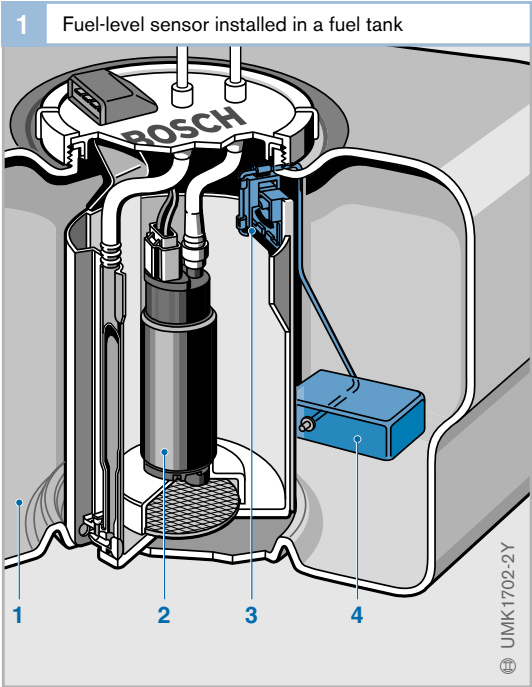
Fig. 1 1 Fuel tank 2 Electric fuel pump 3 Fuel-level sensor 4 Float
