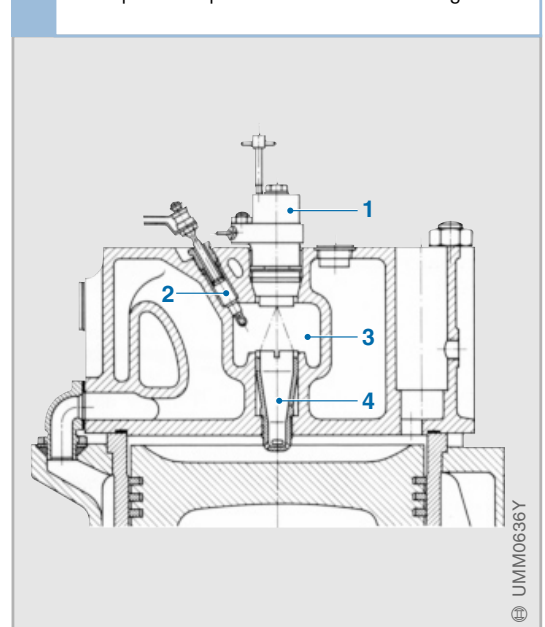
2 Principle of the precombustion-chamber engine
