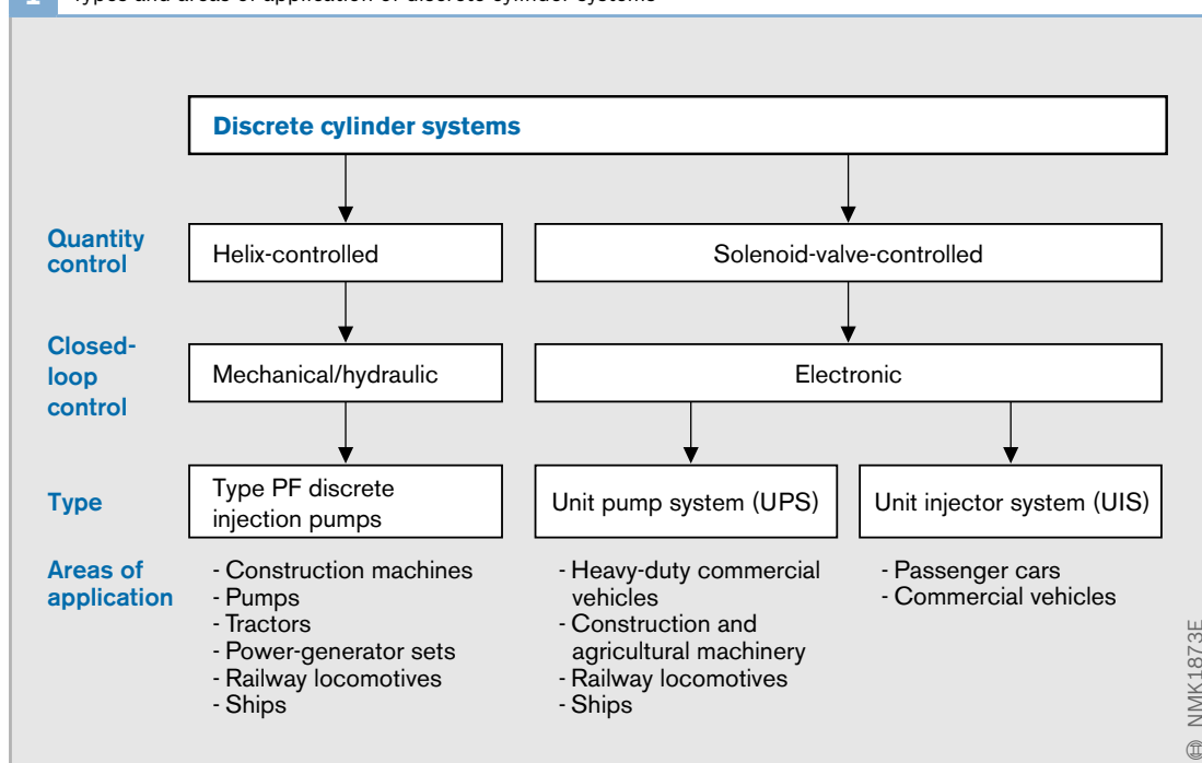
1 Types and areas of application of discrete cylinder systems
