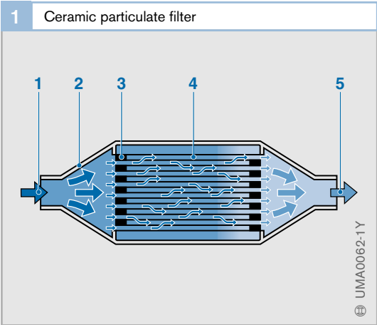
Fig. 1 1 Inflowing exhaust gas 2 Housing 3 Ceramic plug 4 Honeycomb ceramic 5 Outflowing exhaust gas
