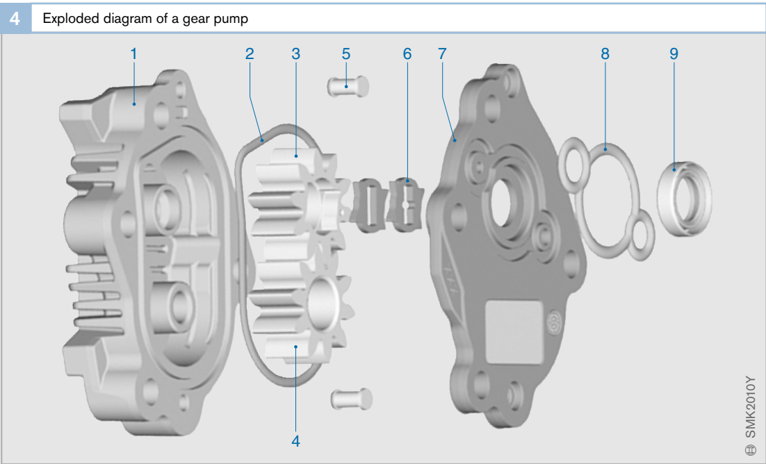
Fig. 4 1 Pump housing 2 O-ring seal 3 Primary gearwheel 4 Secondary gearwheel 5 Rivet 6 Coupling 7 Cover plate 8 Molded seal 9 Shaft seal
