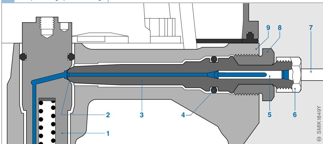
3 Sample of a high-pressure fitting
