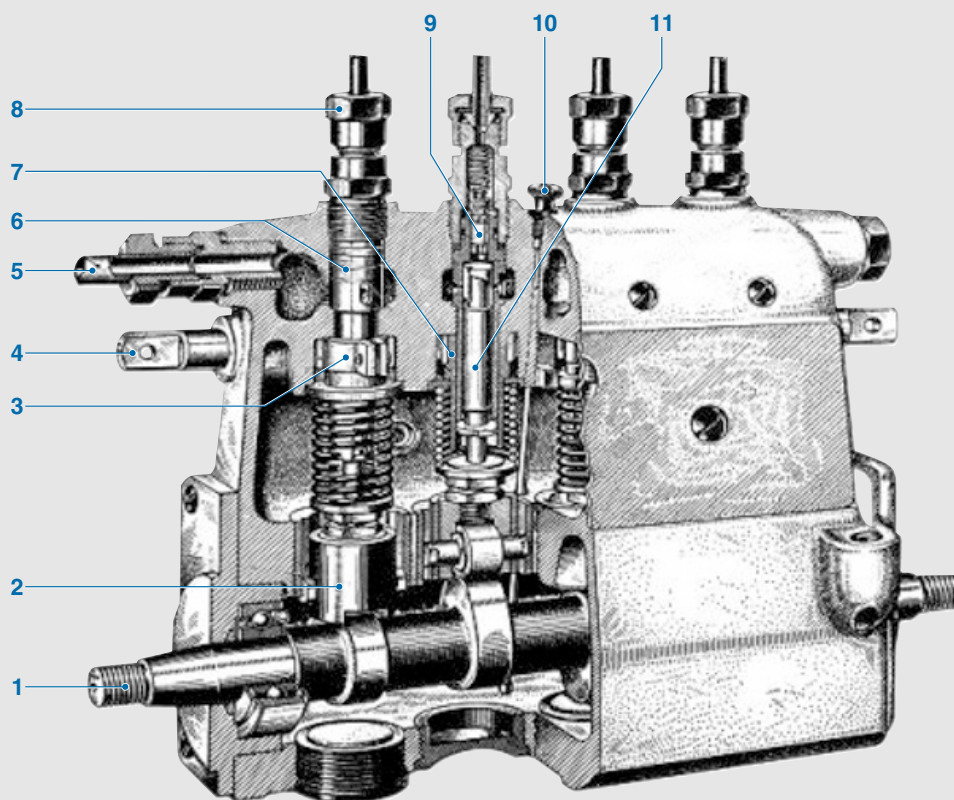
3 First series-production diesel fuel-injection pump from Bosch (1927)
