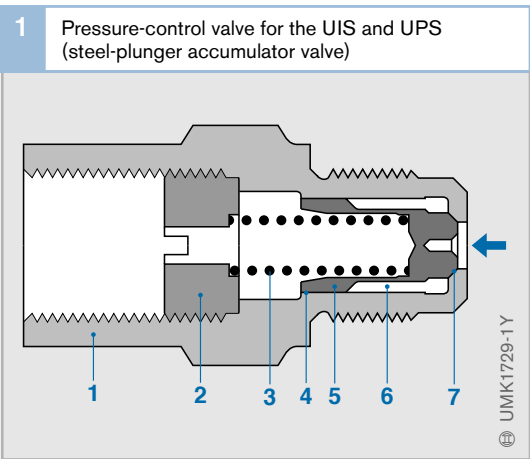
Fig. 1 1 Valve body 2 Threaded element 3 Spring 4 Gap seal 5 Accumulator plunger 6 Accumulator volume 7 Conical seat
