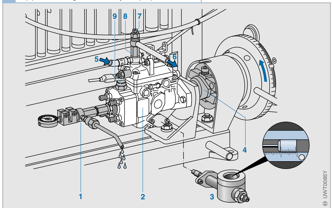
1 Equipment for testing the distributor injection pump (on test bench)
