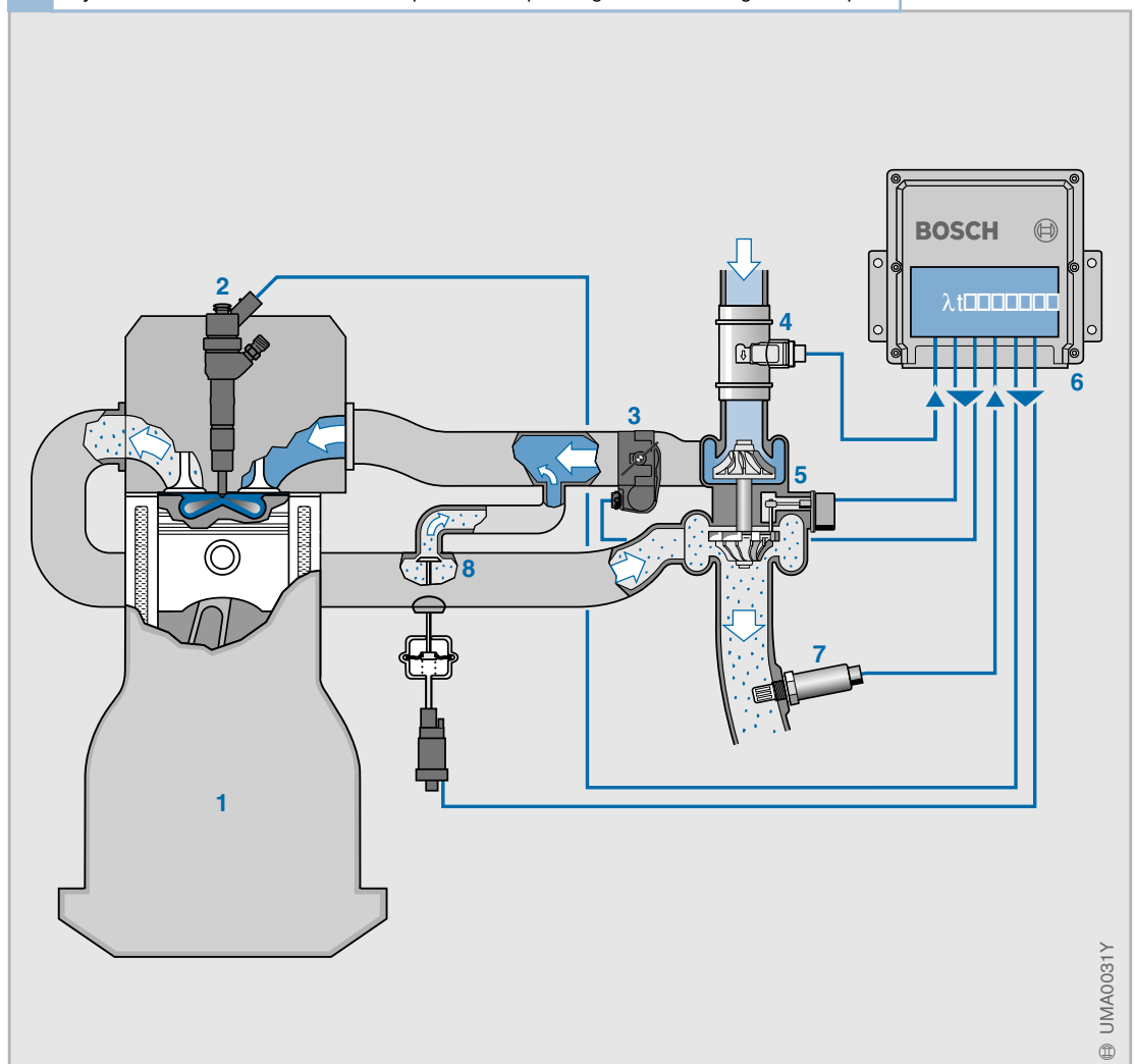
1 System overview of lambda closed-loop control for passenger-car diesel engines (example)
