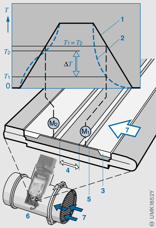
3 Hot-film air-mass meter: Measuring principle
