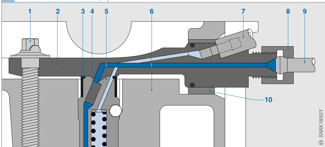
4 Sample of a perpendicular fitting
