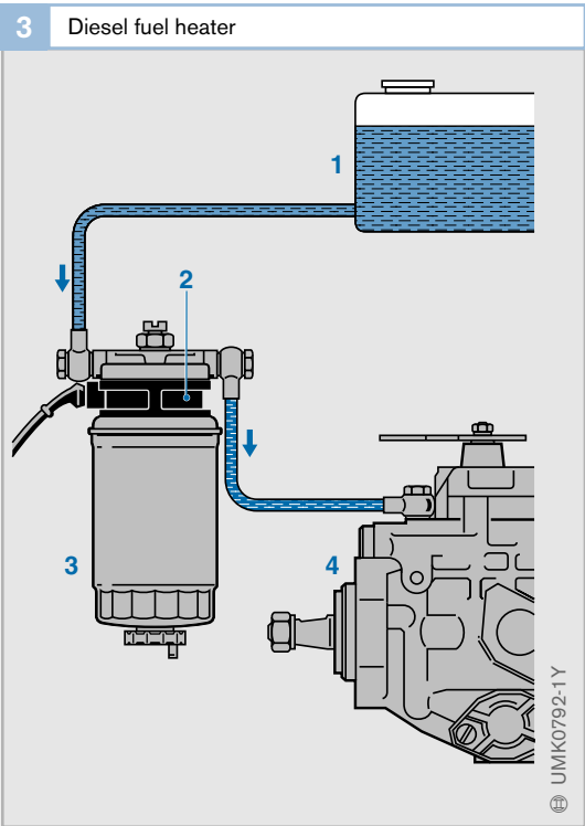
Fig. 3 1 Fuel tank 2 Fuel heater 3 Fuel filter 4 Fuel-injection pump
