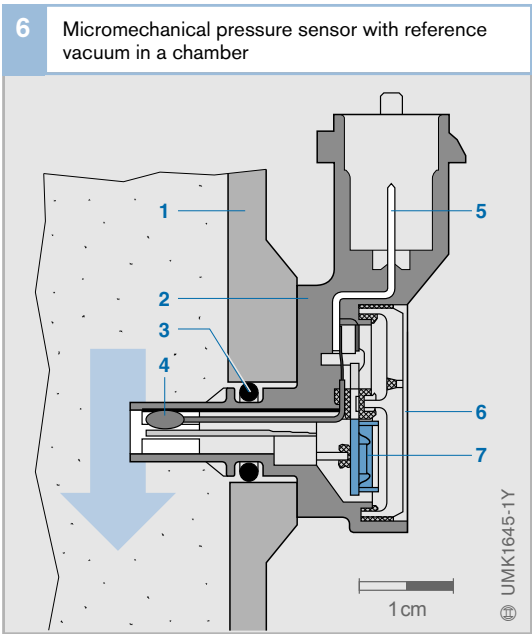
Fig. 6 1 Manifold wall 2 Case 3 Seal ring 4 Temperature sensor (NTC) 5 Electrical connection (socket) 6 Case cover 7 Measuring element
