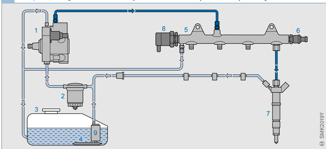
3 Example of a third-generation common-rail system with two-actuator system for a 4-cylinder engine
