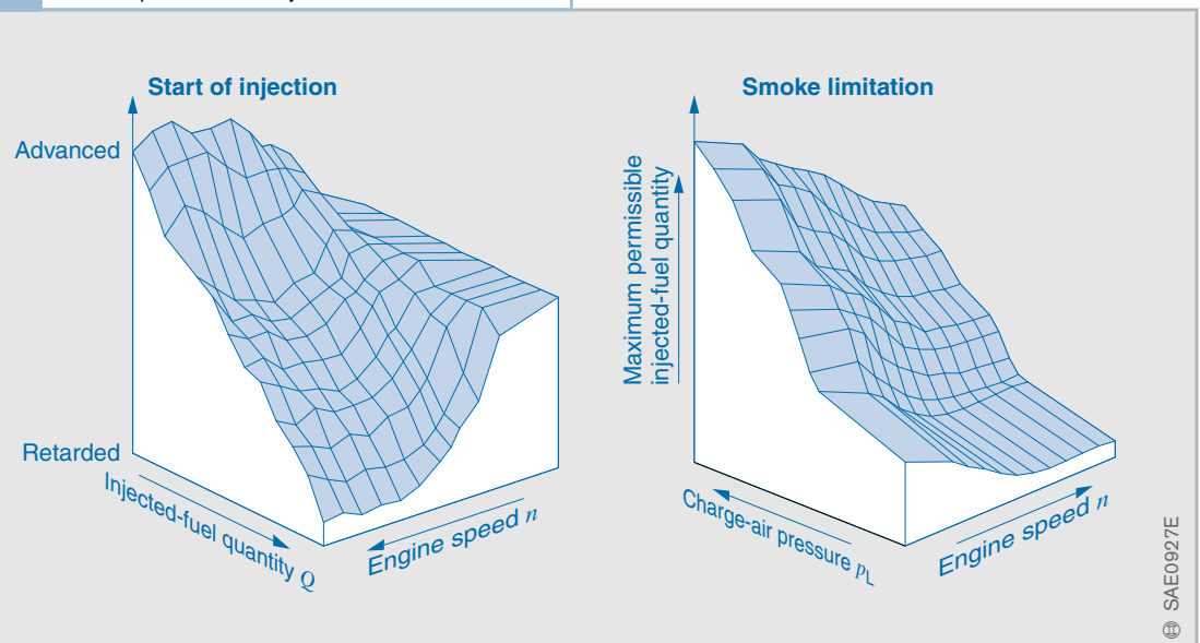
3 Data maps for start of injection and smoke limitation
