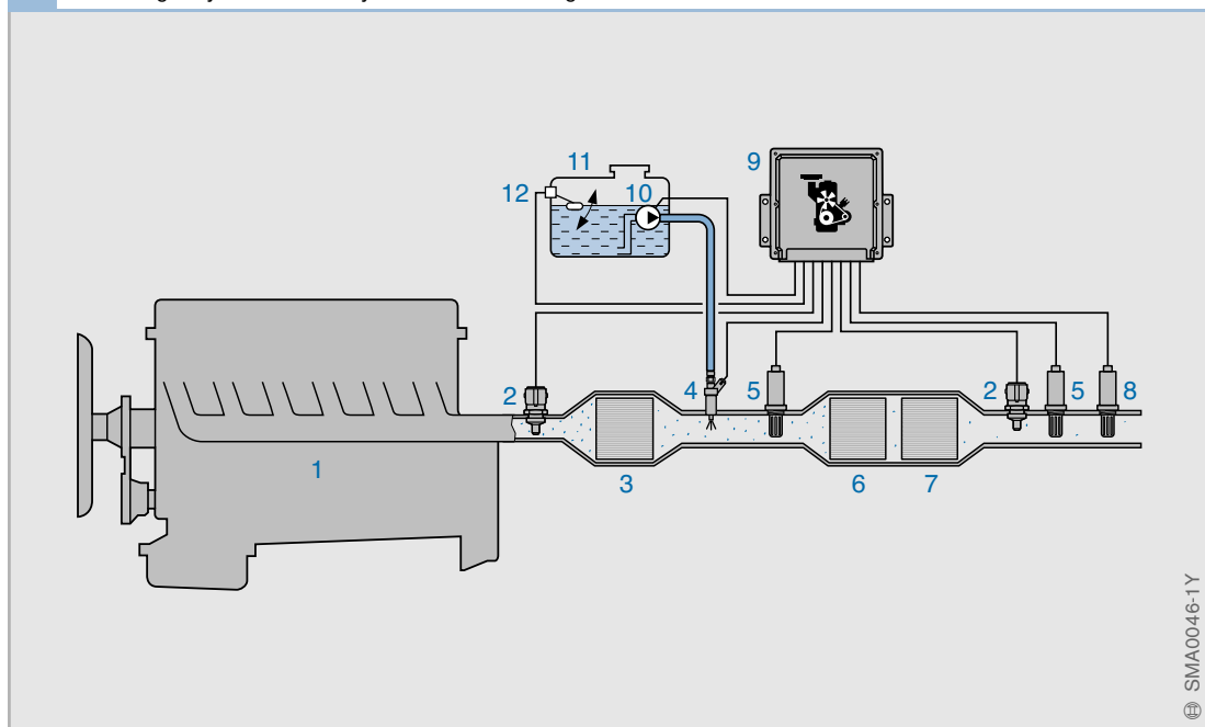
1 Exhaust-gas system with catalytic reduction of nitrogen oxides (SCR)
