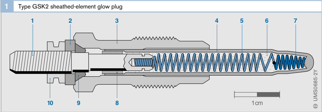
Fig. 1 1 Connector 2 Insulating washer 3 Body 4 Element sheath 5 Control filament 6 Magnesium oxide powder 7 Heating filament 8 Element seal 9 Double seal 10 Knurled nut
