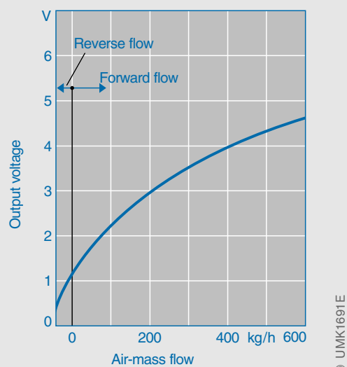
2 Hot-film air-mass meter (output voltage as a function of the partial air mass flowing past it)
