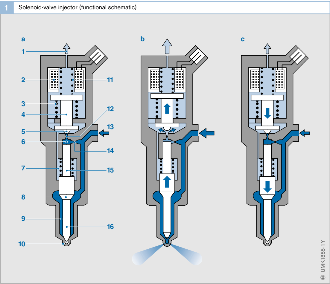
Fig. 1 a Resting position b Injector opens c Injector closes 1 Fuel-return 2 Solenoid coil 3 Overstroke spring 4 Solenoid armature 5 Valve ball 6 Valve-control chamber 7 Nozzle spring 8 Pressure shoulder of nozzle needle 9 Chamber volume 10 Injection orifice 11 Solenoid-valve spring 12 Outlet restrictor 13 High-pressure connection 14 Inlet restrictor 15 Valve plunger (control plunger) 16 Nozzle needle
