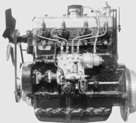
Bosch in-line fuel-injection pump on the engine of the Mercedes 260D
