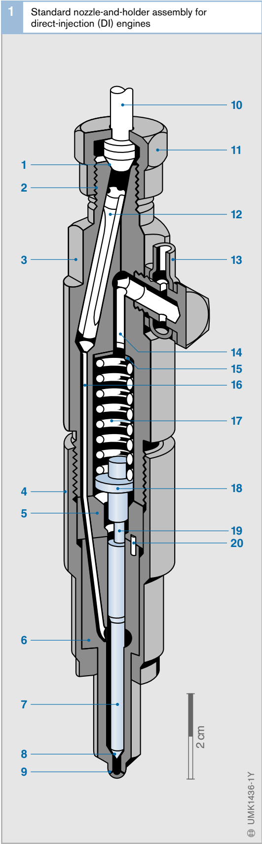
Fig. 1 1 Sealing cone 2 Screw thread for central pressure connection 3 Holder body 4 Nozzle-retaining nut 5 Intermediate disk 6 Nozzle body 7 Nozzle needle 8 Nozzle-body seat face 9 Injection orifice 10 Fuel inlet 11 Sleeve nut 12 Edge-type filter 13 Leak fuel connection 14 Leak fuel port 15 Shim 16 Pressure passage 17 Compression spring 18 Pressure pin 19 Pressure pin 20 Locating pin
