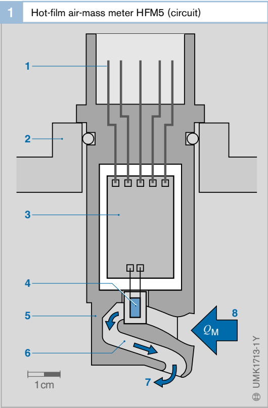
Fig. 1 1 Electrical plug-in connection 2 Measuring tube or air-filter housing wall 3 Evaluation electronics (hybrid circuit) 4 Sensor element 5 Sensor housing 6 Partial-flow measuring tube 7 Air outlet for the partial air flow Q_M 8 Intake for partial air flow Q_M
