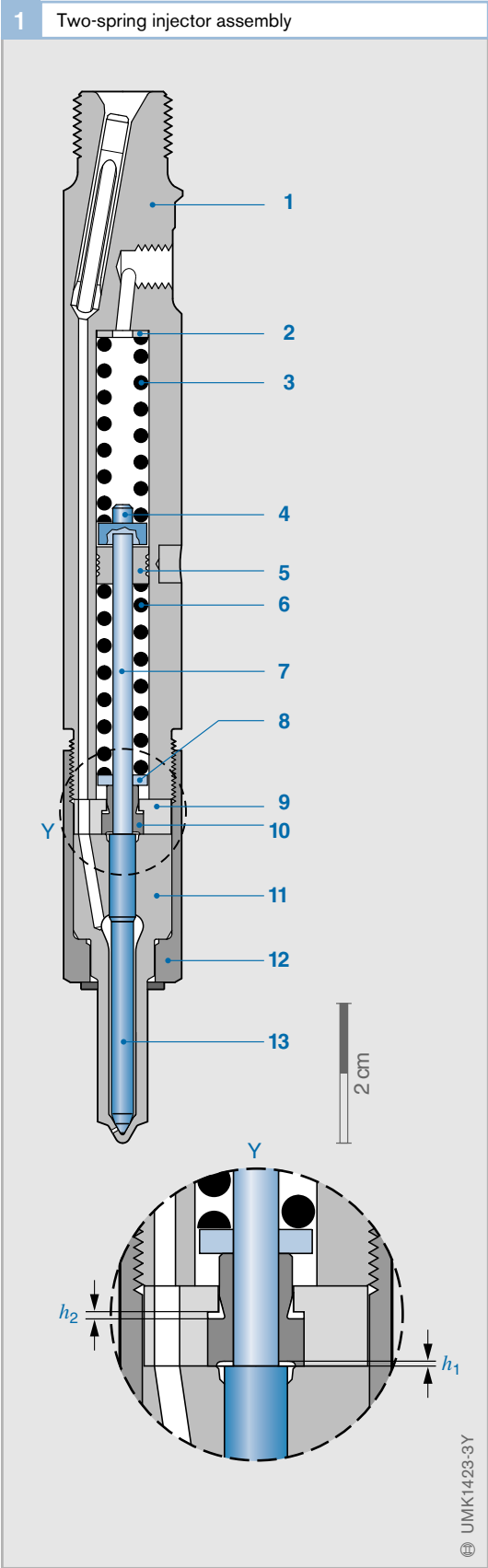
Fig. 1 1 Holder body 2 Shim 3 Compression spring 1 4 Pressure pin 5 Guide washer 6 Compression spring 2 7 Pressure pin 8 Spring seat 9 Intermediate disk 10 Stop sleeve 11 Nozzle body 12 Nozzle-retaining nut 13 Nozzle needle h_1 Plunger lift to port closing h_2 Main lift
