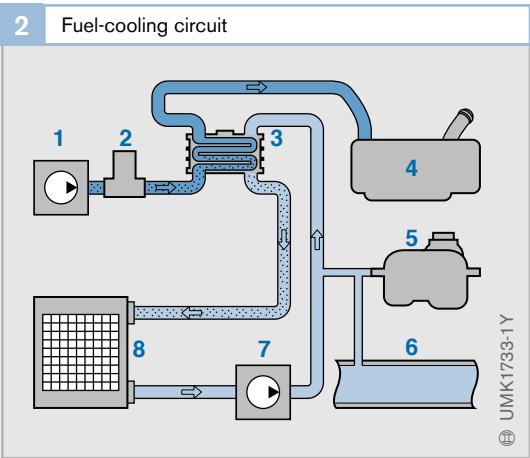
Fig. 2 1 Fuel pump 2 Fuel-temperature sensor 3 Fuel cooler 4 Fuel tank 5 Equalizing reservoir 6 Engine-cooling circuit 7 Coolant pump 8 Auxiliary cooler
