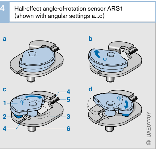
Fig. 4 1 Rotor (permanent magnet) 2 Pole shoe 3 Conductive element 4 Air gap 5 Hall-effect sensor 6 Shaft (magnetically soft) \varphi Angle of rotation
