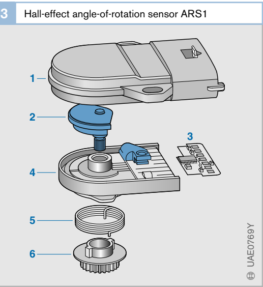
Fig. 3 1 Housing cover 2 Rotor (permanent magnet) 3 Evaluation electronics with Hall-effect sensor 4 Housing base 5 Return spring 6 Coupling element (e.g. gear)
