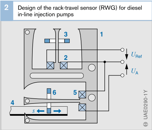
Fig. 2 1 Soft-iron core 2 Reference coil 3 Reference short-circuiting ring 4 Control rack 5 Measuring coil 6 Measuring short-circuiting ring s Control-rack travel Fig. 3 U_A Output voltage U_{Ref} Reference voltage
