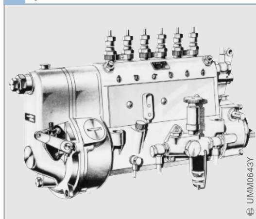
4 Bosch fuel-injection pump with mounted mechanical governor
