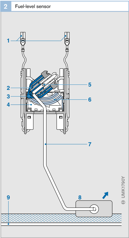
Fig. 2 1 Electrical connections 2 Wiper spring 3 Contact rivet 4 Resistor board 5 Bearing pin 6 Twin contact 7 Float lever 8 Float 9 Fuel-tank floor
