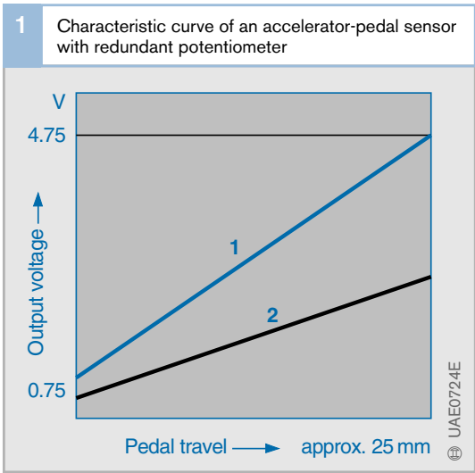
Fig. 1 1 Potentiometer 1 (master potentiometer) 2 Potentiometer 2 (50% of voltage)
