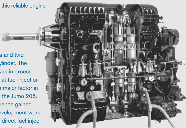
▼ Junkers Jumo 205 two-stroke opposed-piston diesel aircraft engine
